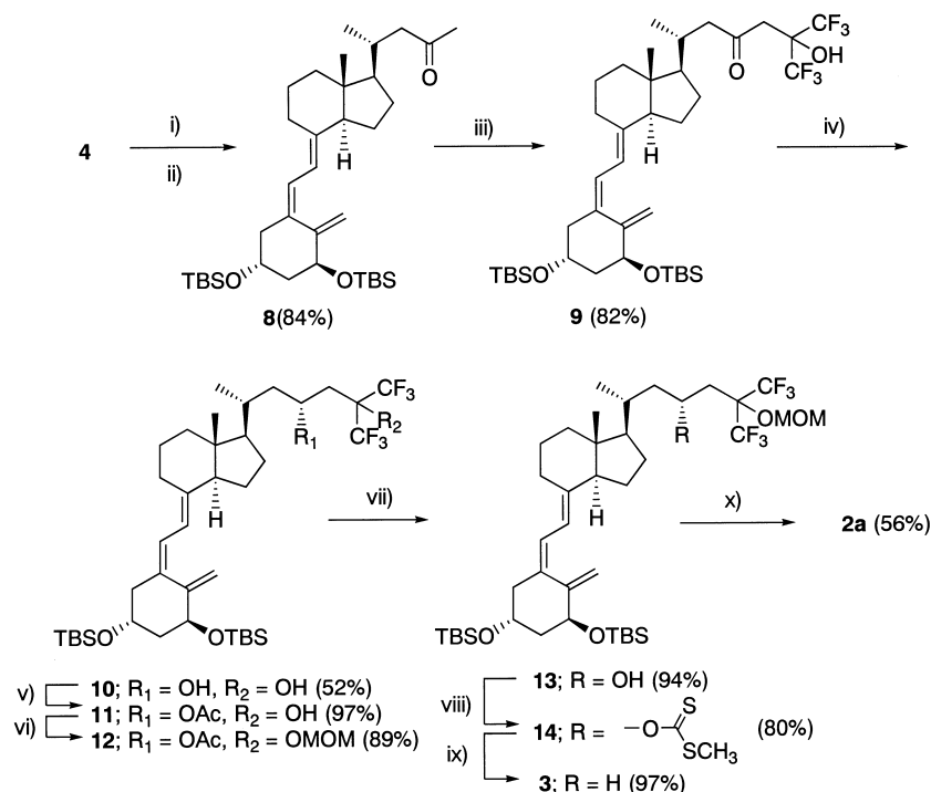
Scheme 2. The preparation of 2a from 4 . (i) MeMgBr, Et 2 O, 0 °C, 30 min; (ii) TPAP, NMO, MS4A, CH 2 Cl 2 , rt, 15 min; (iii) CF 3 COCF 3 , LiN(TMS) 2 , THF, –70 °C, 30 min; (iv) NaBH 4 , THF–MeOH, –10 °C, 10 min; (v) Ac 2 O, pyridine, rt, 12 h; (vi) MOMCl, i Pr 2 NEt, CHCl 3 , reflux, 1 h; (vii) KOH–MeOH, 0 °C, 1 h; (viii) NaH, CS 2 , rt, overnight then CH 3 I; (ix) nBu 3 SnH, toluene, reflux, 1 h; (x) MsOH, MeOH, rt, 2 h.
