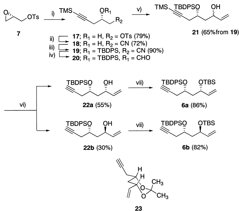
Scheme 4. The preparation of enyne compounds ( 6a , 6b ) from 7 . (i) Trimethylsilylacetylene, n\text{BuLi} , \text{BF}_3 \cdot \text{Et}_2\text{O} , THF, -70^\circ\text{C} ; (ii) KCN, DMSO, 40^\circ\text{C} , 3 h; (iii) TBDPSCl, imidazole, DMF, 40^\circ\text{C} , 2 h; (iv) DIBALH, \text{CH}_2\text{Cl}_2 , -10^\circ\text{C} , 30 min; (v) vinylmagnesium bromide, THF, -70^\circ\text{C} \rightarrow \text{rt} , 30 min; (vi) \text{K}_2\text{CO}_3 , MeOH, rt, 1 h; (vii) TBSCl, imidazole, DMF, 40^\circ\text{C} , 2 h.
