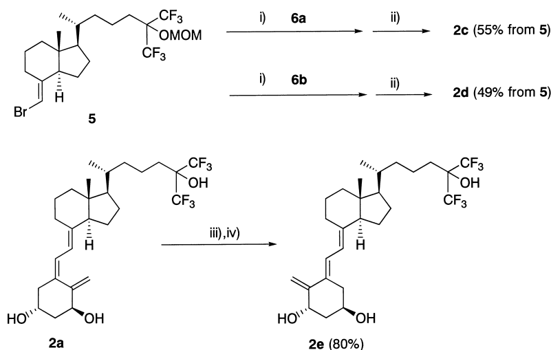
Scheme 6. Synthesis of 2c , 2d , 2e . (i) (\text{dba})_3\text{Pd}_2\cdot\text{CHCl}_3 , \text{NEt}_3 , toluene, reflux, 10 min; (ii) \text{MsOH} , \text{MeOH} , rt, 1 h; (iii) liquified \text{SO}_2 , \text{CH}_2\text{Cl}_2 , reflux, 30 min; (iv) \text{NaHCO}_3 , \text{EtOH} , reflux, 90 min.
