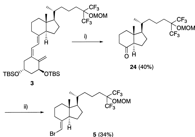
Scheme 5. Preparation of the CD ring fragment 5 from 3 . (i) \text{O}_3 , \text{PPh}_3 , -78^\circ\text{C} , 30 min; (ii) \text{LiN}(\text{TMS})_2 , bromotriphenylphosphonium bromide, toluene, -78^\circ\text{C} , 30 min.
