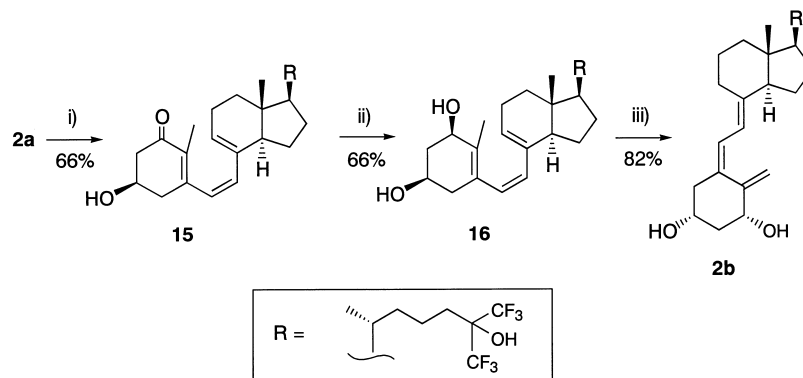
Scheme 3. The preparation of 1-epimer 2b from 2a . (i) Dess–Martin periodinane, CH 3 CN, rt, 4 h; (ii) NaBH 4 , MeOH, 0 °C, 1.5 h; (iii) acetone, 80 °C, 6 h.
