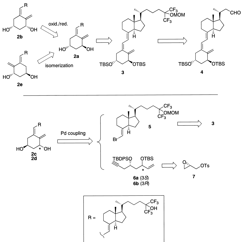
Scheme 1. Synthetic plan for the synthesis of A-ring isomers of 2a .
